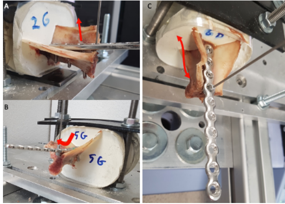
Figure 1. Modes of failure: (A) DCP pull through, (B) PLS plate bending, (C) PLS scapula bending.
