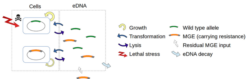
FIG 1 Schematic representation of the computational model. Bacterial cell growth follows a logistic growth model. The bacterial cells have an insertion site in their chromosome at which two types of alleles from the eDNA compartment can be integrated from transformation and replace their current DNA: wild-type (WT) allele and MGE. The integration of a WT allele is costless for cells, whereas the integration of MGEs causes a cost in terms of cell replication. Bacterial populations are faced with stochastic stresses of random duration and intensity. In the absence of stress, cells are lysed at a basal rate. Under stress exposure, the lysis rate of WT cells increases but remains unchanged for cells with an MGE carrying resistance. Each lysed cell releases its DNA and fuels the extracellular compartment with eDNA. MGEs are constantly added to the extracellular environment at a marginal rate (MGE input) simulating residual arrival from neighboring populations. The WT alleles and MGEs are degraded at a constant rate in the extracellular compartment.
